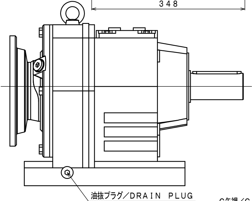
C矢視/C-VIEW
