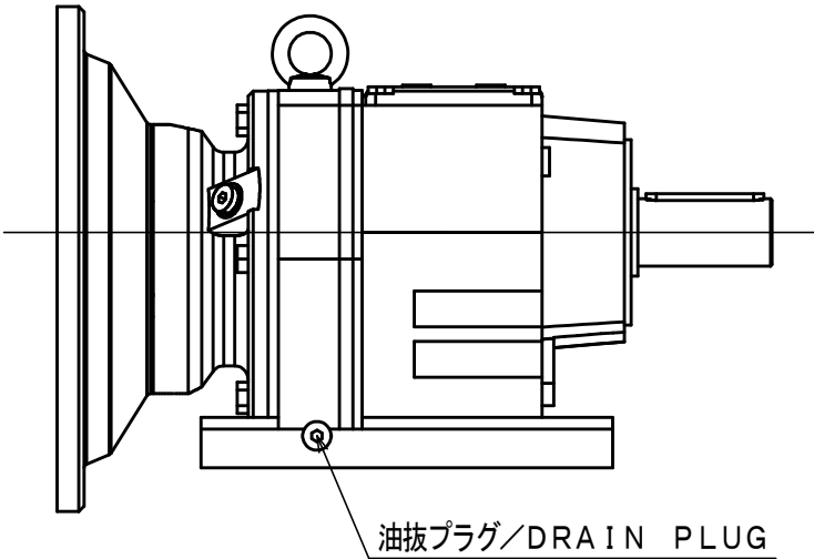
C矢視/C-View
