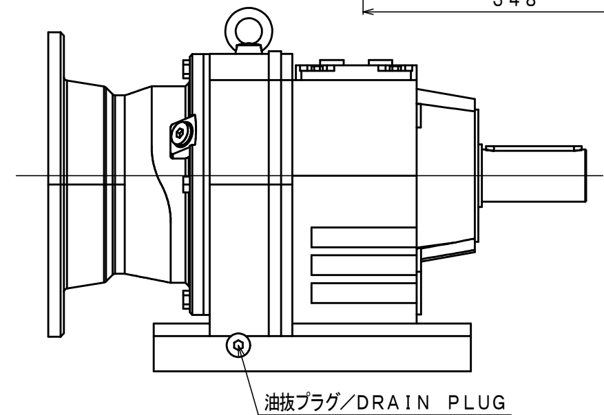
C矢視／C-View
